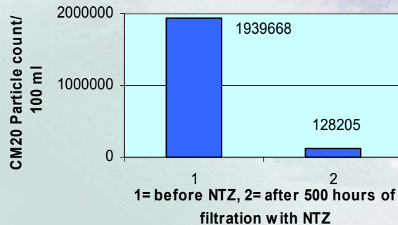
Particles > 2 micron
