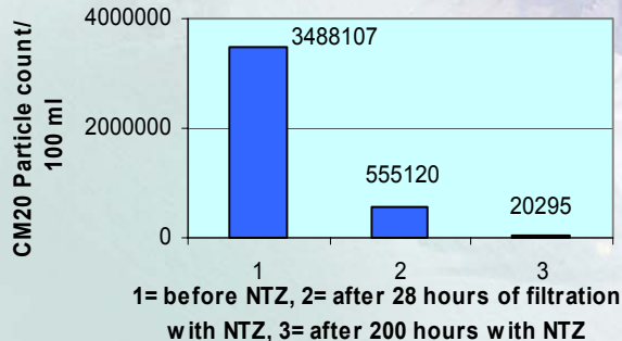
Particles > 2 micron
